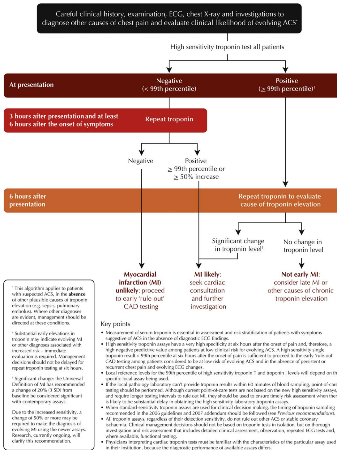
Figure 1. Algorithm for incorporating a high sensitivity troponin into the work-up of patients with suspected acute coronary syndromes (ACS).
